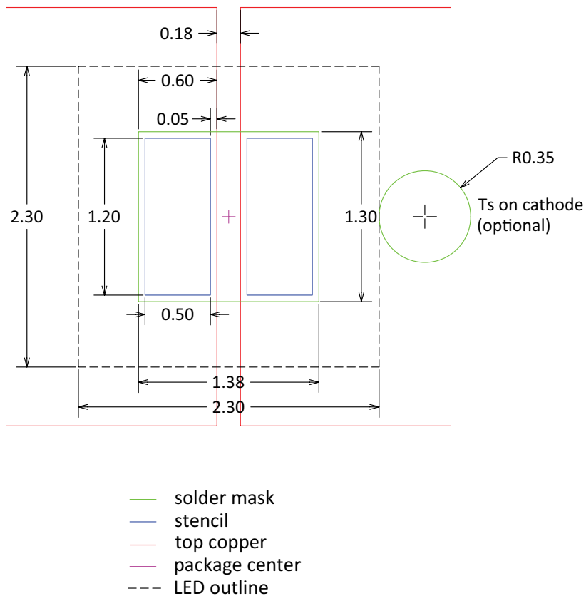
Figure 19. Recommended PCB solder pad layout for LUXEON HL2Z.
