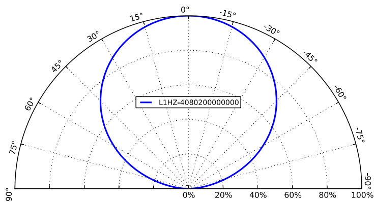
Figure 14. Typical polar radiation pattern for LUXEON HL2Z at 700mA, T_j=85^{\circ}\text{C} .
