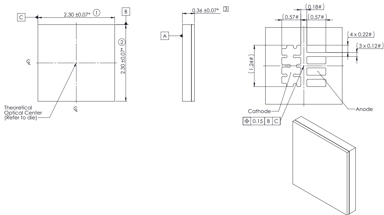
Figure 17. Mechanical dimensions for LUXEON HL2Z.
