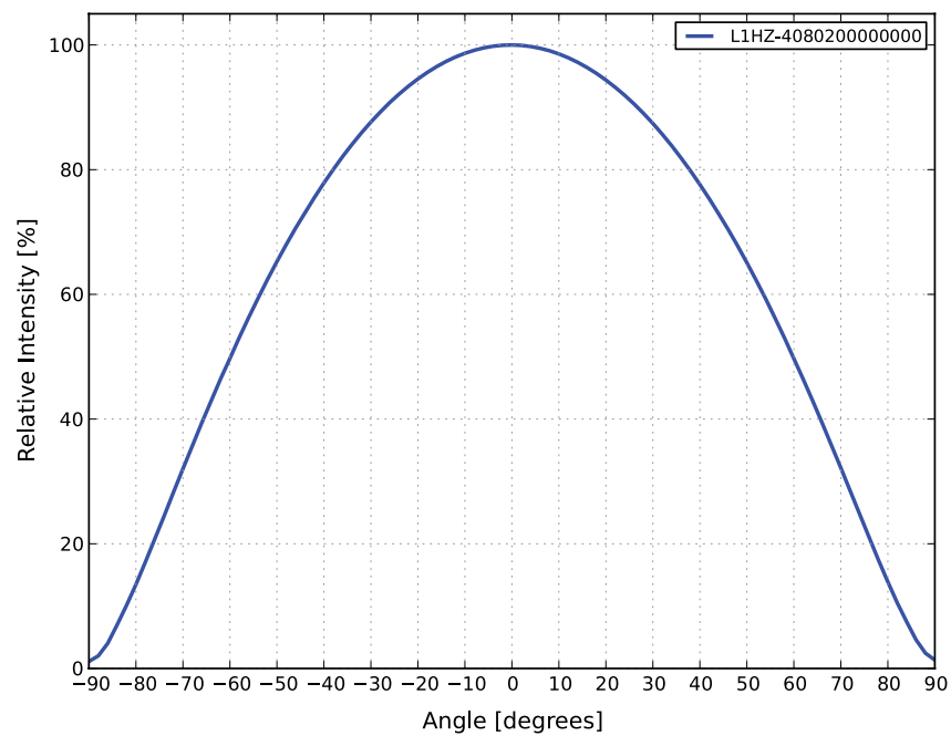
Figure 13. Typical radiation pattern for LUXEON HL2Z at 700mA, T_j=85^{\circ}\text{C} .
