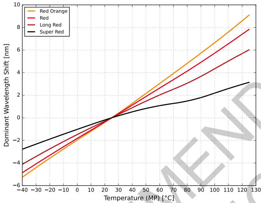
Figure 1b. Typical dominant wavelength shift vs junction temperature for SignalSure 30 at 20 ms MP, 30 mA, T_j = 25\text{ °C}
