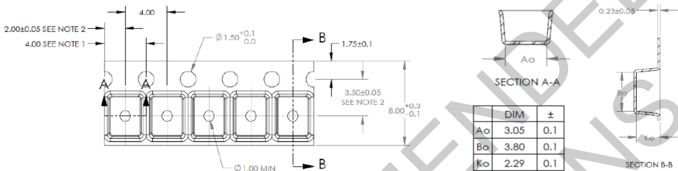
Figure 11. Pocket tape dimensions for SignalSure 30
