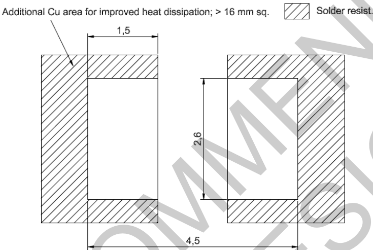
Figure 10. Recommended PCB solder pad layout for SignalSure 30
