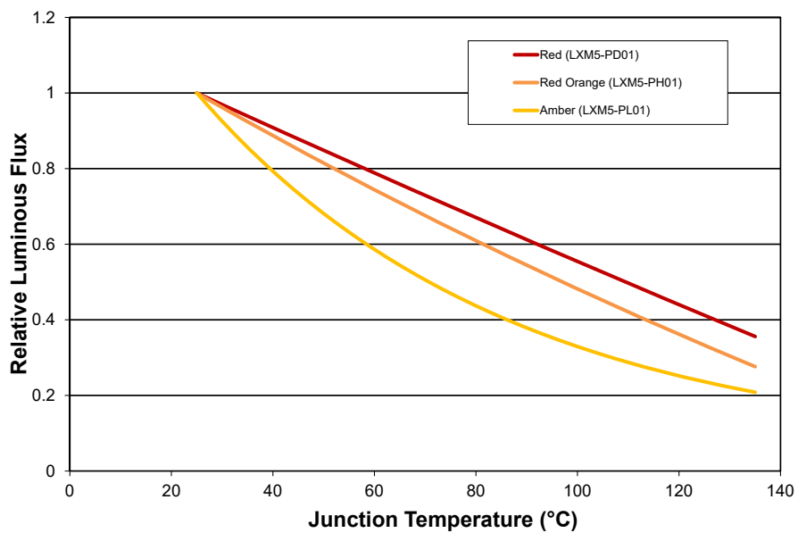
Figure 2c. Typical normalized light output vs. junction temperature for LXM5-PD01, LXM5-PH01 and LXM5-PL01 at test current.
