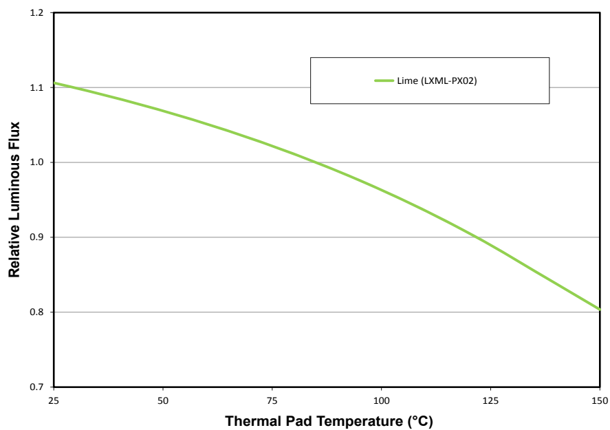
Figure 2d. Typical normalized light output vs. junction temperature for LXML-PX02 at test current.
