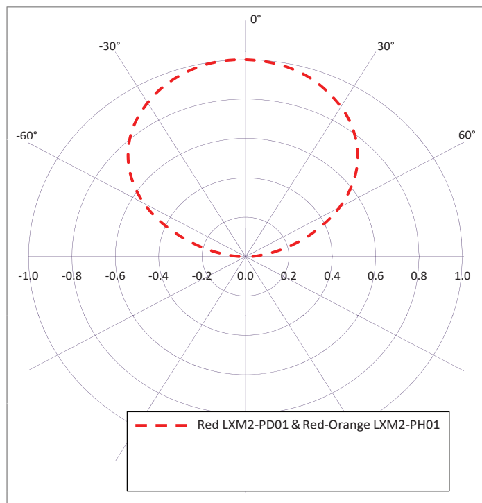
Figure 5b. Typical polar radiation pattern for LXM2-PD01 and LXM2-PH01 at test conditions.
