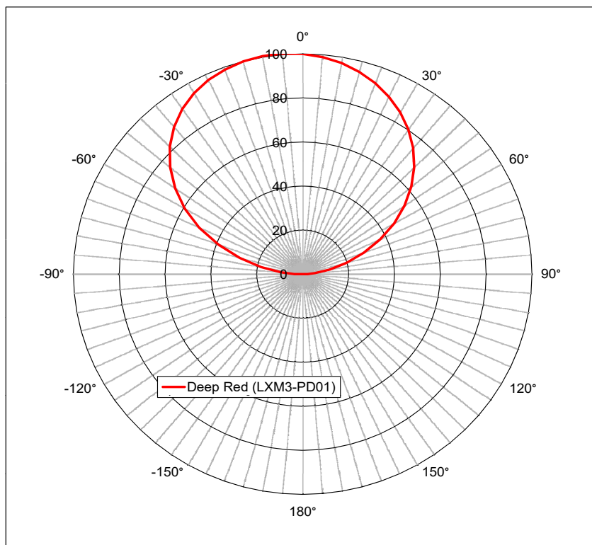
Figure 5c. Typical polar radiation pattern for LXM3-PD01 at test conditions.
