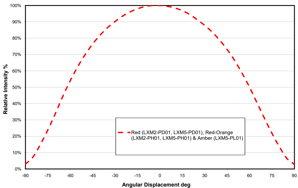
Figure 4b. Typical radiation pattern for LXM2-PD01, LXM5-PD01, LXM2-PH01, LXM5-PH01 and LXM5-PL01 at test conditions.
