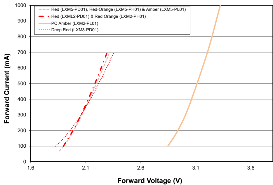
Figure 3b. Typical forward current vs. forward voltage for LXM3-PD01, LXM2-PD01, LXM5-PD01, LXM2-PH01, LXM5-PH01, LXM2-PL01 and LXM5-PL01 at test temperature.
