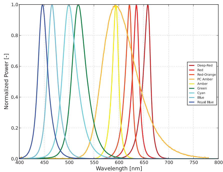
Figure 1a. Typical normalized power vs. wavelength for LUXEON Rebel Deep Red, Red, Red-Orange, PC Amber, Amber, Green, Cyan, Blue and Royal Blue at test current, T_j=25^{\circ}\text{C} .
