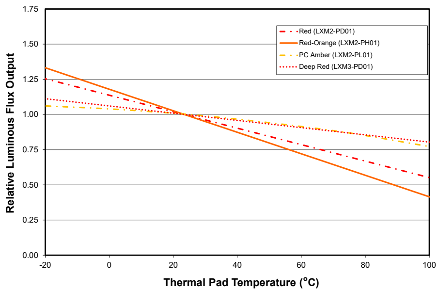
Figure 2b. Typical normalized light output vs. junction temperature for LXM3-PD01, LXM2-PD01, LXM2-PH01, LXM2-PL01, at test current.
