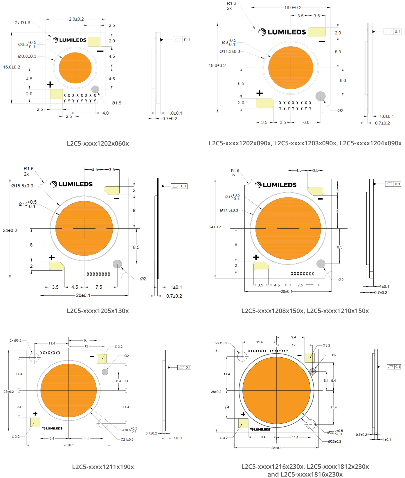
Figure 8. Mechanical dimensions for LUXEON CoB Core Range.
