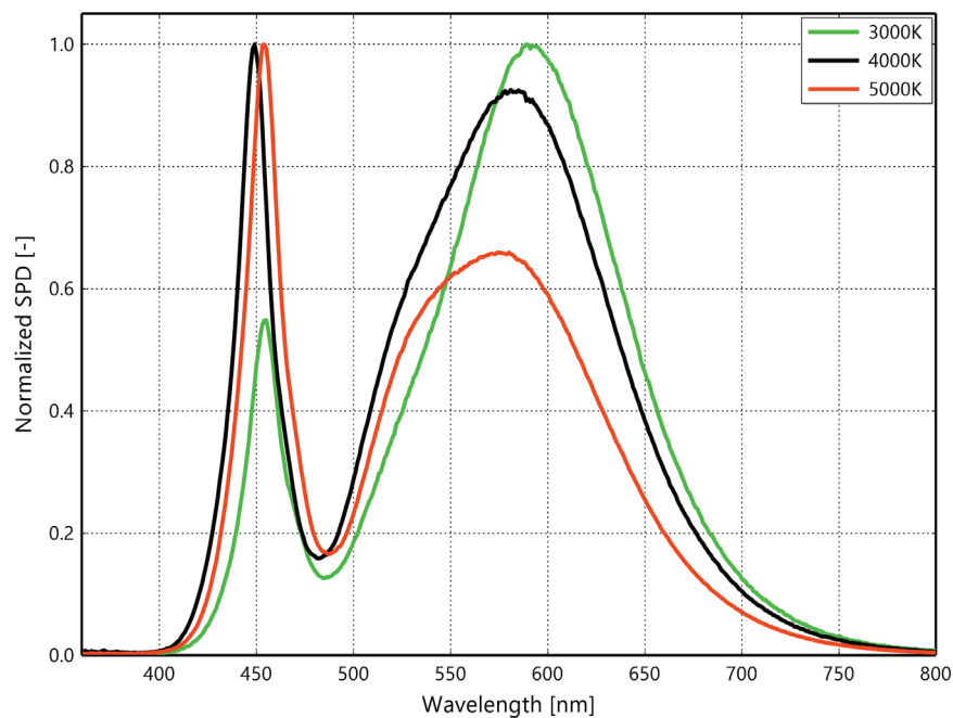
Figure 1a. Typical normalized power vs. wavelength for L2C5-xx70xxxHxx0x at specified test current, T_j=85^{\circ}\text{C} .
