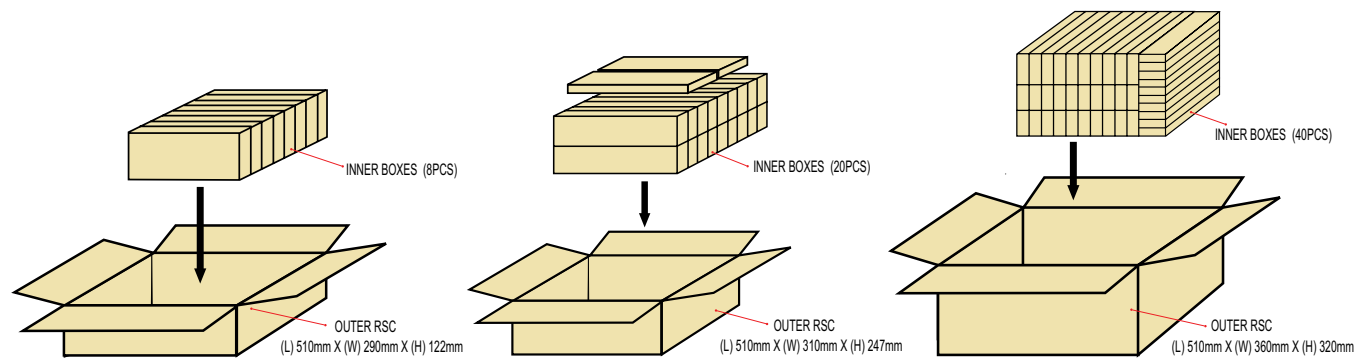
Figure 13. Dimensions for outer box packaging for LUXEON CoB Core Range High Density Gen 2.
