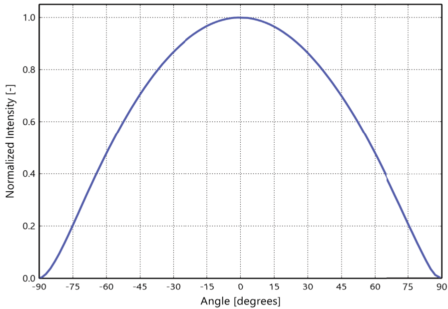
Figure 5. Typical radiation pattern for LUXEON CS Pro CoB at specified test current, T_j=85^{\circ}\text{C} .
