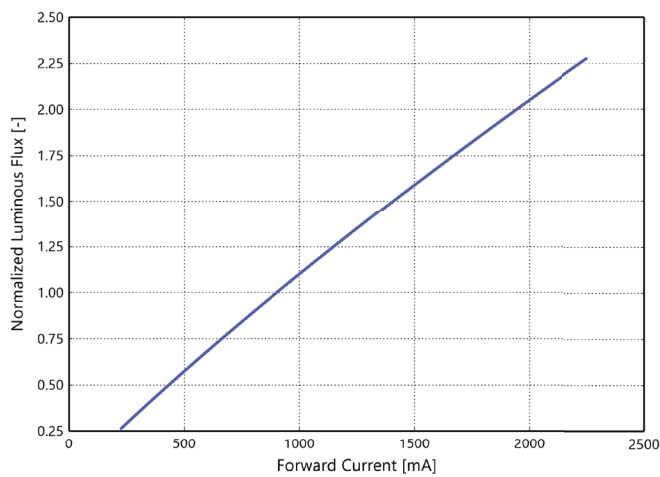
Figure 3b. Typical normalized light output vs. forward current for L2C6-xxxxL10A15X0 at Tj=85°C.
