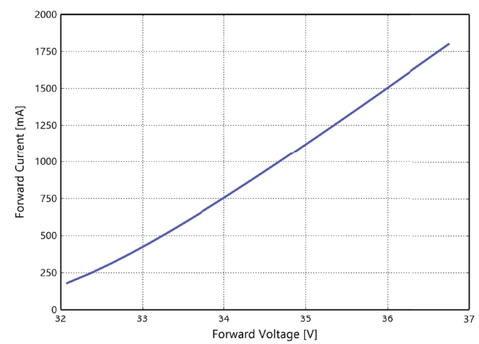
Figure 4a. Typical forward current vs. forward voltage for L2C6-xxxxxL08A15X0 at T_j=85^{\circ}\text{C} .
