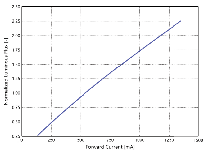
Figure 3f. Typical normalized light output vs. forward current for L2C6-xxxxxL06A1300 at T_j=85^{\circ}\text{C} .
