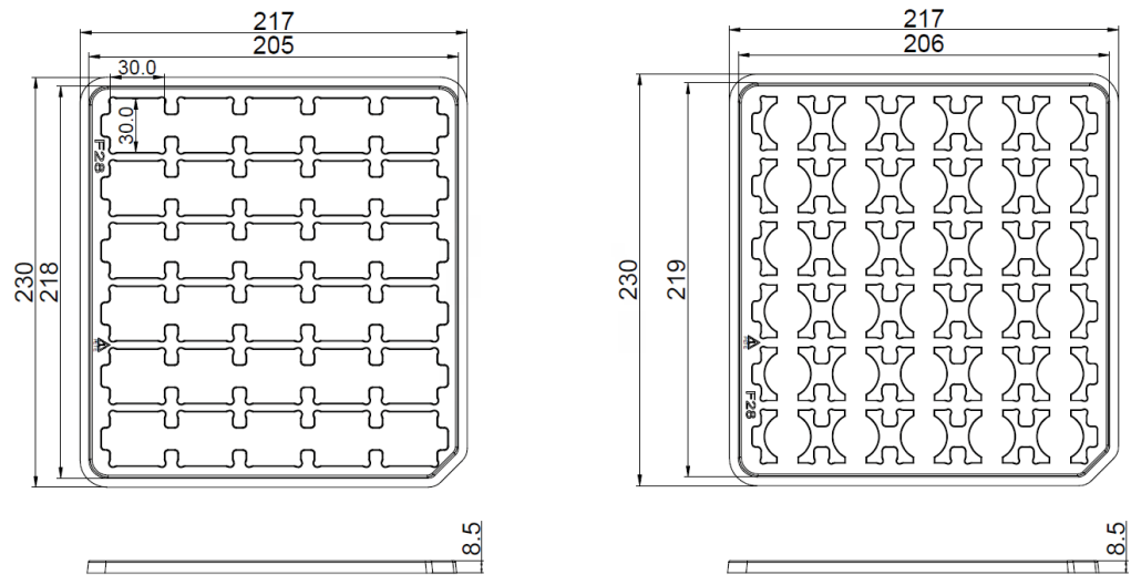
Figure 9c. Tray dimensions for L2C6-xxxxxL11x2200, L2C6-xxxxxL13x2200, L2C6-xxxxxL16x2200, L2C6-xxxxxR12x2200 and L2C6-xxxxxR18x2200.
