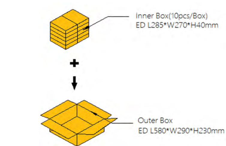
Figure 12. Dimensions for outer box packaging for LUXEON CS CoB.
