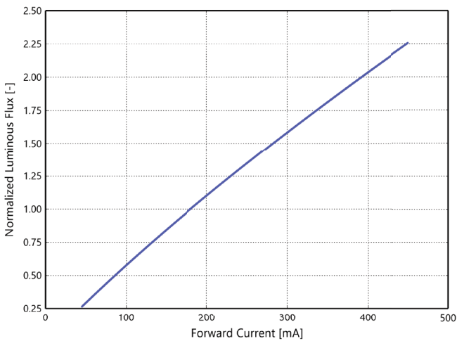
Figure 3b. Typical normalized light output vs. forward current for L2C6-xxxxL02A0900 at T j =85°C.
