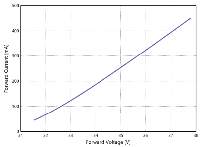
Figure 4b. Typical forward current vs. forward voltage for L2C6-xxxxxL02A0900 at T_j=85^{\circ}\text{C} .
