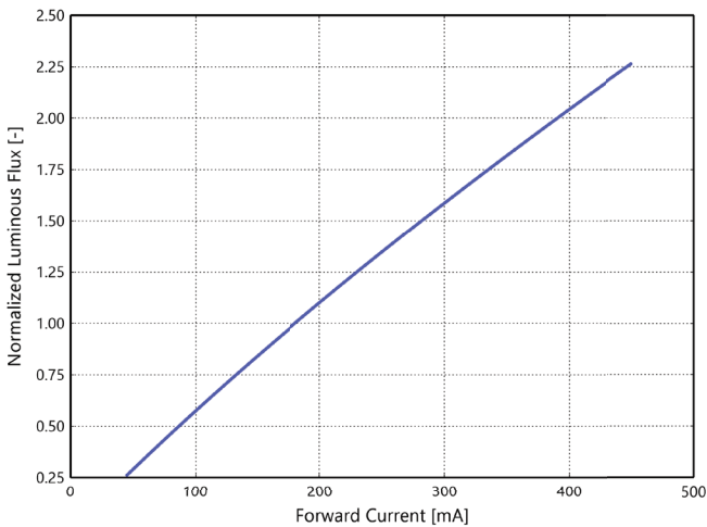
Figure 3a. Typical normalized light output vs. forward current for L2C6-xxxxL02A0600 at T j =85°C.
