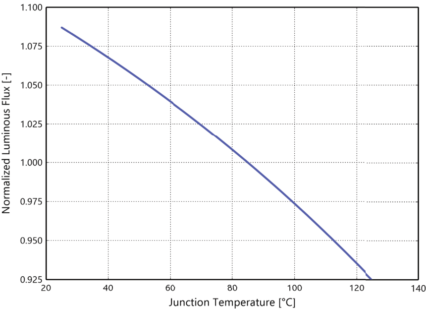
Figure 2. Typical normalized light output vs. junction temperature for L2C6-xxxxLxxAxx00 at specified test current.
