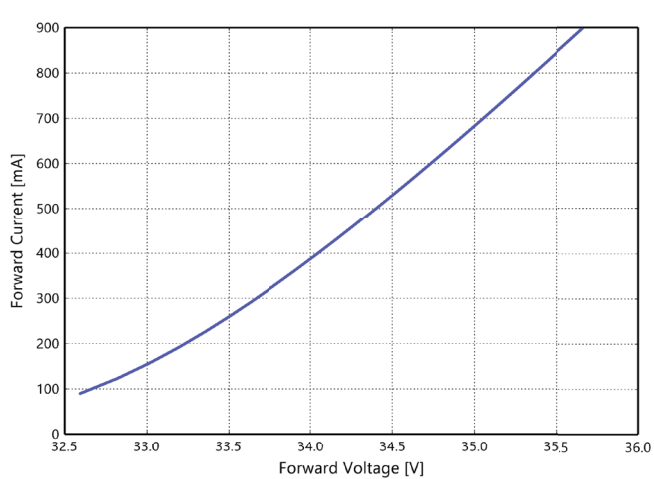
Figure 4d. Typical forward current vs. forward voltage for L2C6-xxxxxL04A0900 at T_j=85^{\circ}\text{C} .
