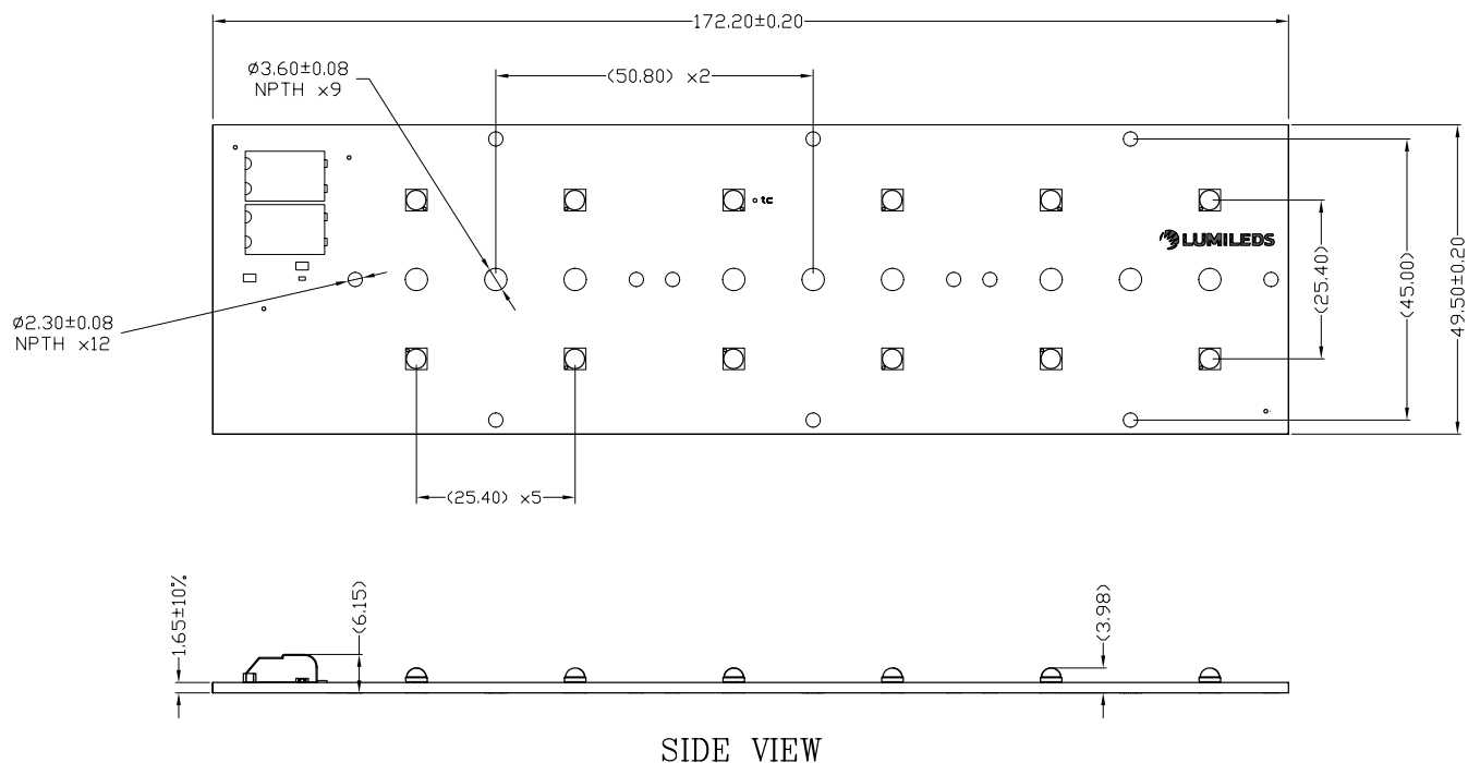
Figure 9. Mechanical dimensions for L213-xxxx012MDE001.
