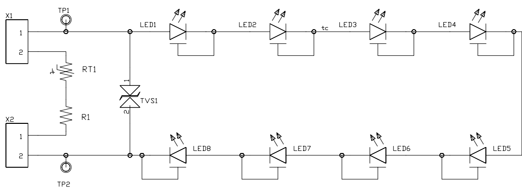
Figure 7. Electric circuit diagram for L2H2-xxxx008MLU010.
