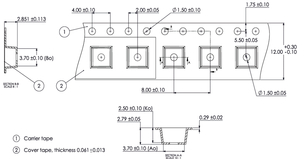
Figure 10. Pocket tape dimensions for LUXEON SunPlus HPE.
