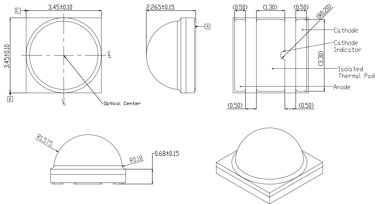
Figure 7. Mechanical dimensions for LUXEON SunPlus HPE.
