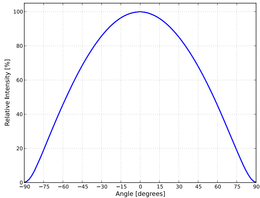
Figure 5. Typical radiation pattern for LUXEON CoB Core Pro at specified test current, T_j=85^{\circ}\text{C} .
