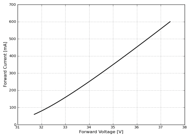
Figure 4b. Typical forward current vs. forward voltage for L2C5-xxxx1203XxxBx at T_j=85^{\circ}\text{C} .
