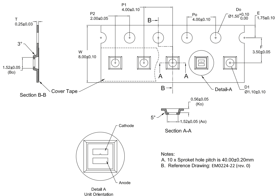
Figure 12. Pocket tape dimensions for LUXEON HL1Z.
