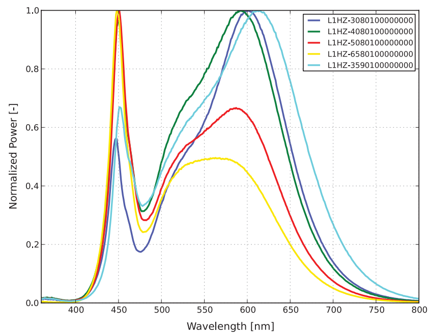
Figure 1. Typical normalized power vs. wavelength for HL1Z at 350mA, T j =85°C.
