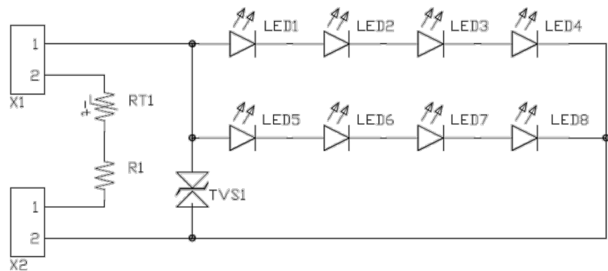
Figure 7. Electric circuit diagram for L213-xxxx008MRH001.
