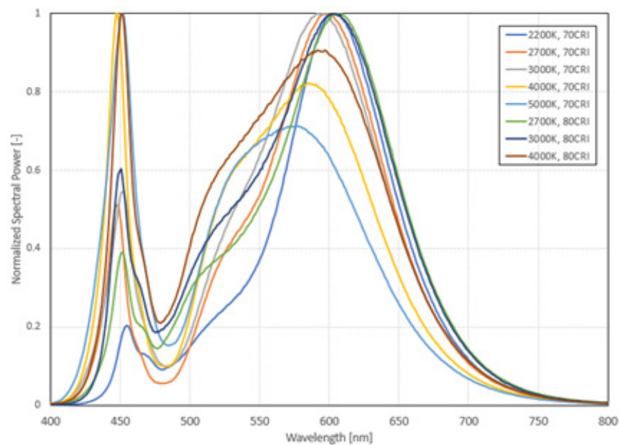
Figure 1a. Typical normalized spectral power vs. wavelength for LUXEON XR-5050 SQR at 700mA, T c =85°C.
