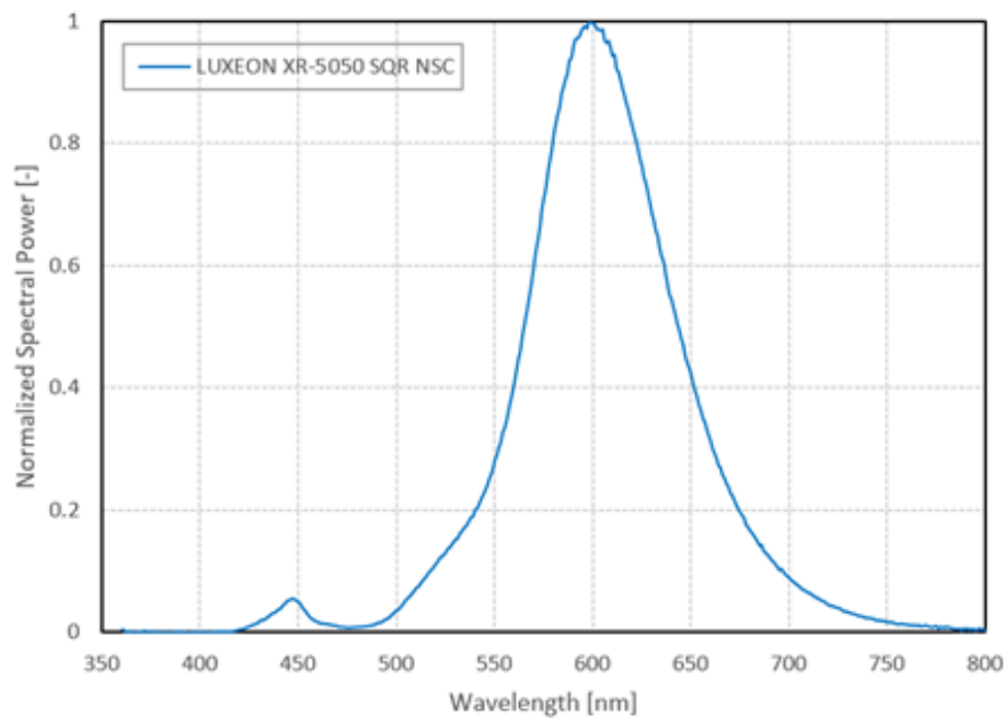
Figure 1b. Typical normalized spectral power vs wavelength for L213-NSC1XXXMRH001 at 700mA, T c =85°C.
