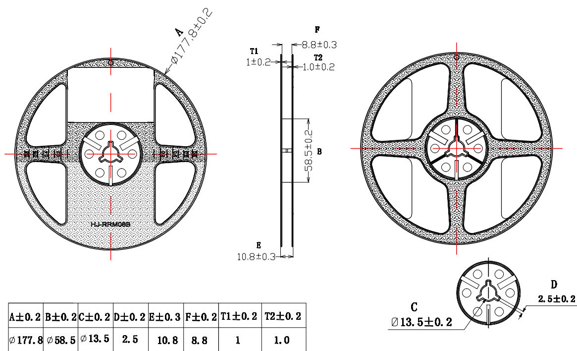
Figure 20. Reel dimensions for LUXEON 2835 Color Line.
