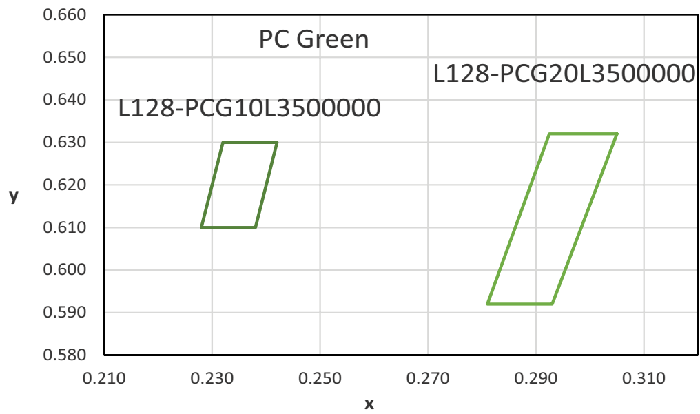
Figure 13. Color Bin Structure for LUXEON 2835 Color 36V PC Green for Table 8.
