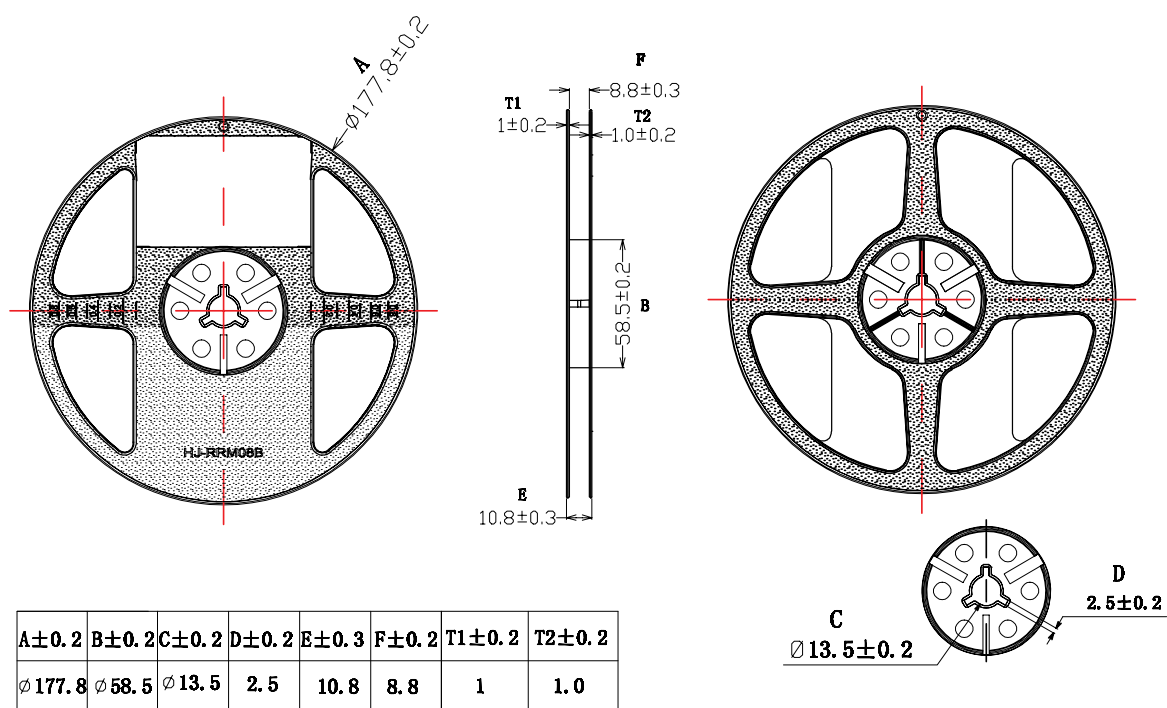
Figure 16. Reel dimensions for LUXEON 2835 Color Line.
