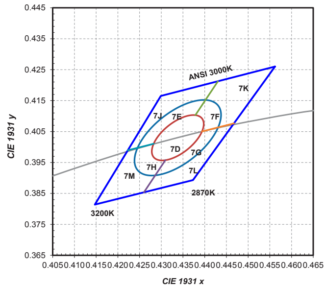
Figure 11a. 1/9 th color bin structure for LUXEON 2835 White 3000K at test current and binning temperature of T_j=25^{\circ}\text{C} .
