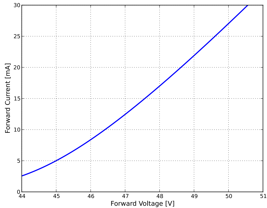
Figure 4b. Typical forward current vs. forward voltage for L130-XXXX0CHV00001 at T j =25°C.
