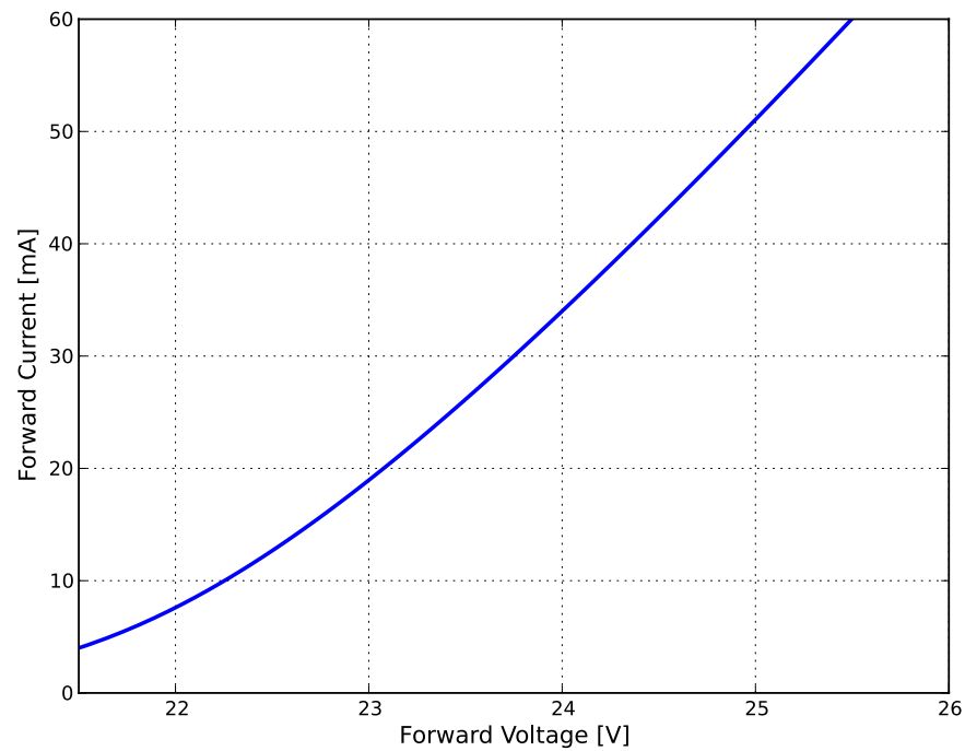
Figure 4a. Typical forward current vs. forward voltage for L130-XXXX0BHV00001 at T j =25°C.
