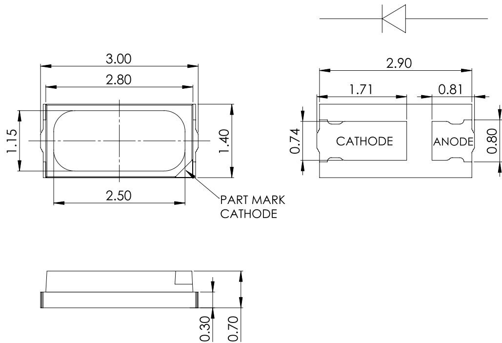
Figure 9. Mechanical dimensions for LUXEON 3014.
