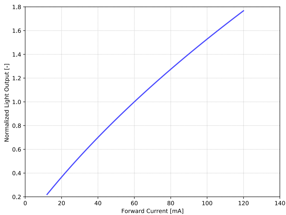
Figure 3. Typical normalized light output vs. forward current for L130-xxxxxx1400001 at T j =25°C.
