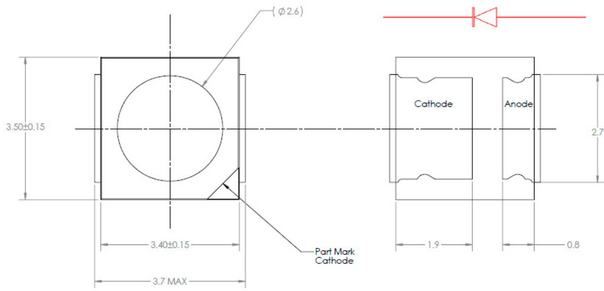
Figure 1. Mechanical dimensions for LUXEON 3535L MXAx-PWxx-S001.
