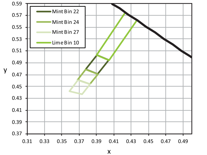
Figure 8. Color bin structure for LUXEON CZ Mint and Lime for Table 7.
