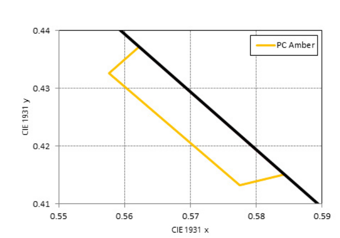
Figure 7. Color bin structure for LUXEON CZ PC Amber for Table 7.
