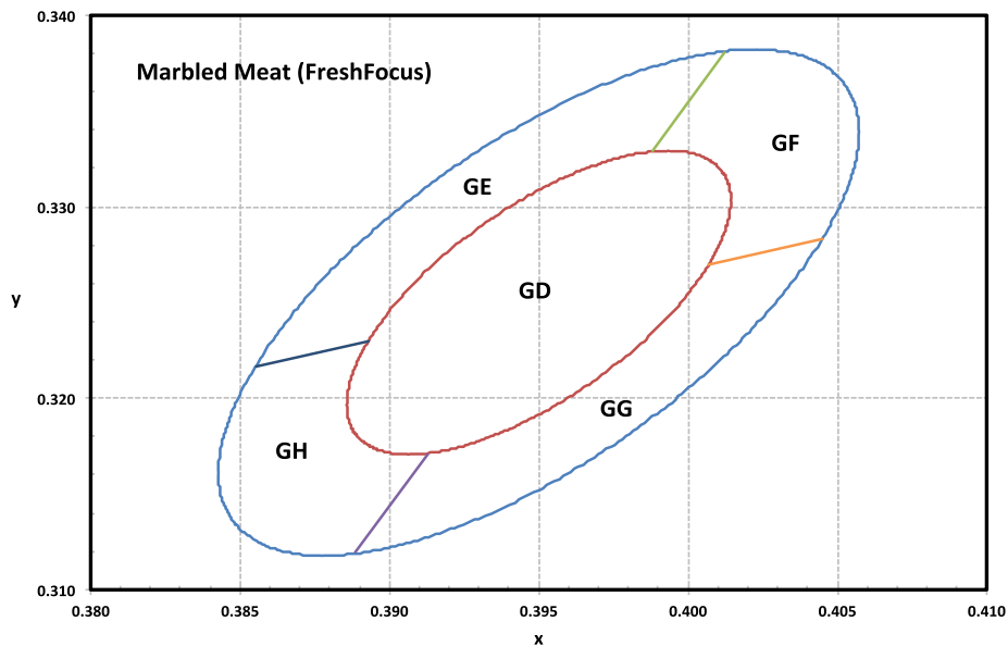
Figure 8c. 1/5 th color bin structure for LUXEON 2835 with FreshFocus Technology for Marbled Meat, 120mA, T_j=25^\circ\text{C} .
