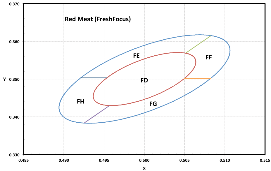
Figure 8b. 1/5 th color bin structure for LUXEON 2835 with FreshFocus Technology for Red Meat, 120mA, T_j=25^\circ\text{C} .
