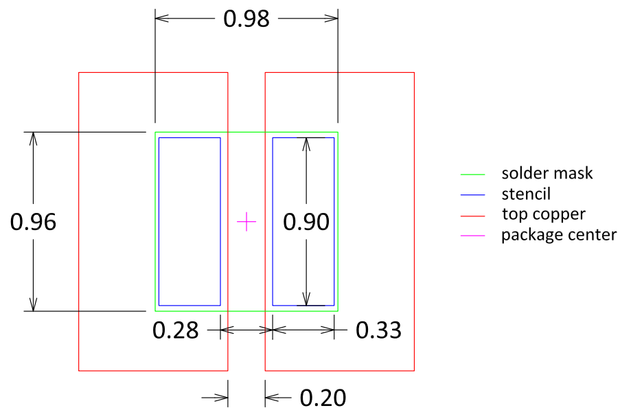
Figure 12. Recommended PCB solder pad layout for LUXEON CSP HL1.
