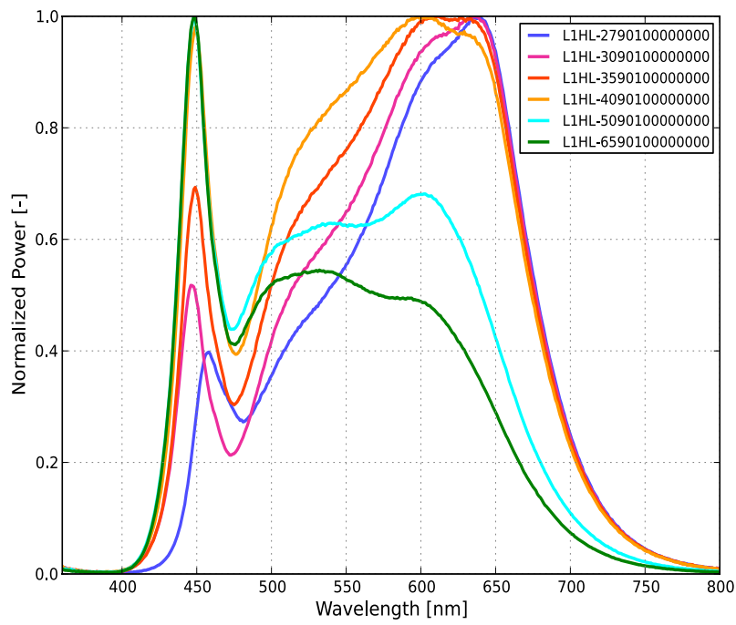
Figure 2. Typical normalized power vs. wavelength for L1HL-xx90100000000 at 350mA, T_j=85^{\circ}\text{C} .
