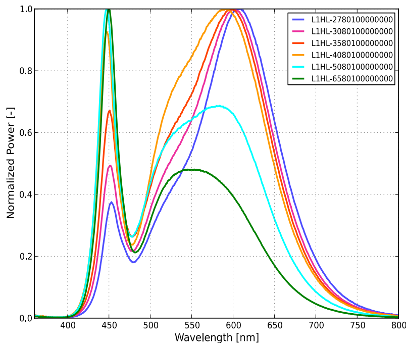
Figure 1. Typical normalized power vs. wavelength for L1HL-xx80100000000 at 350mA, T_j=85^\circ\text{C} .
