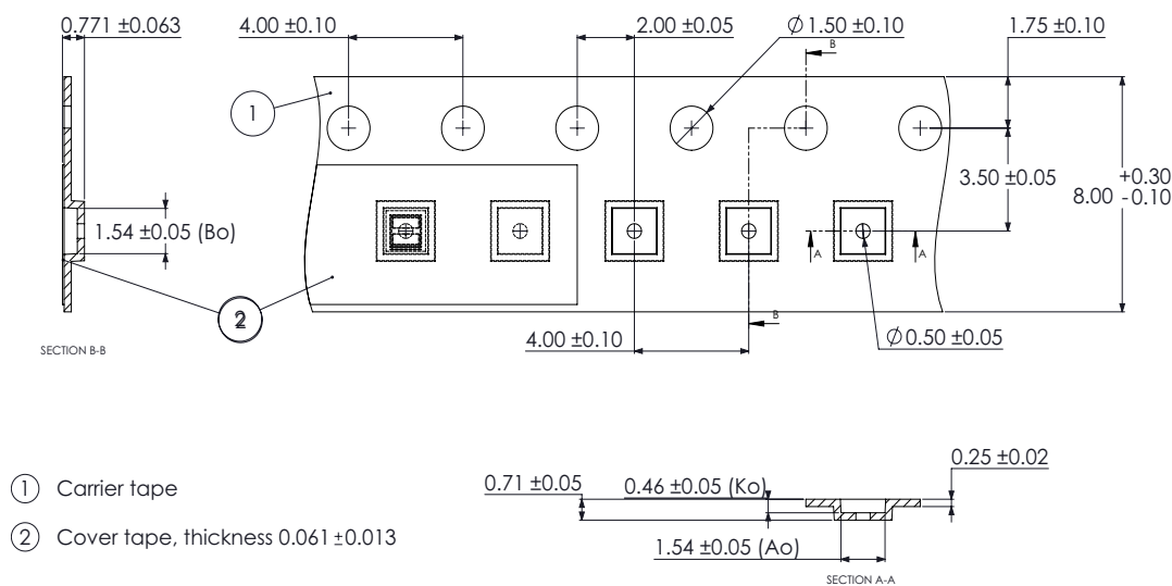
Figure 13. Pocket tape dimensions for LUXEON CSP HL1.
