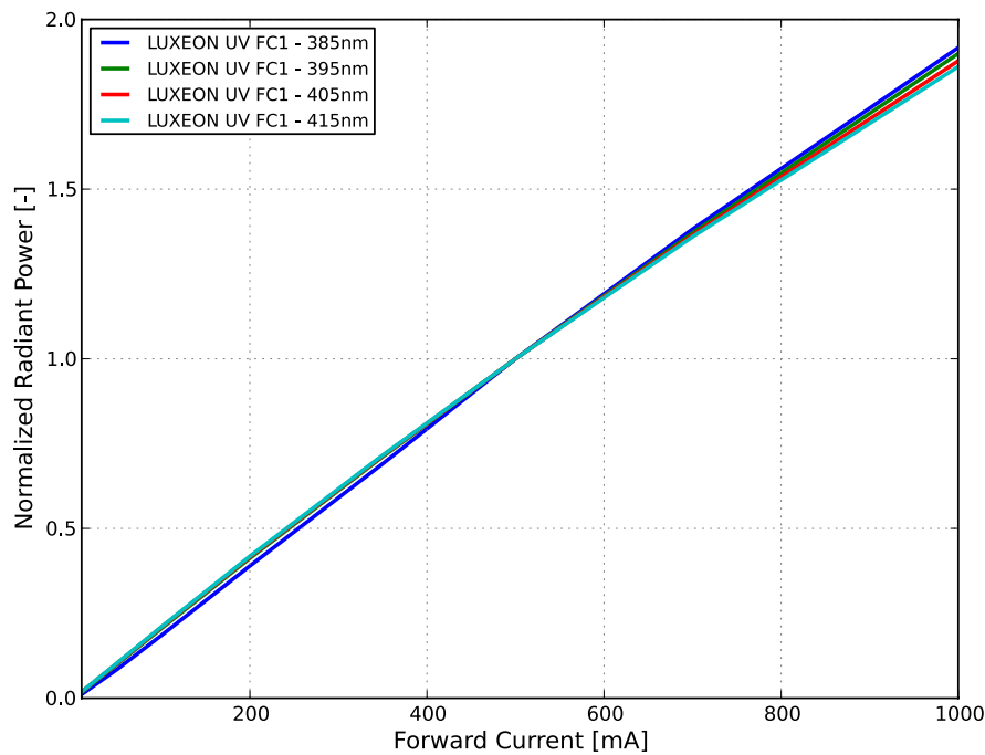
Figure 3. Typical normalized radiant power vs. forward current for LUXEON UV FC Line at T_j=25^{\circ}\text{C} .
