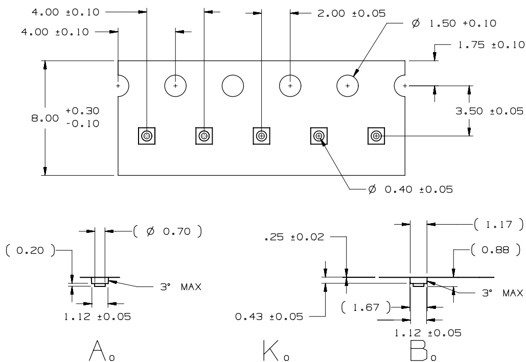
Figure 13. Pocket tape dimensions for LUXEON UV FC Line.
