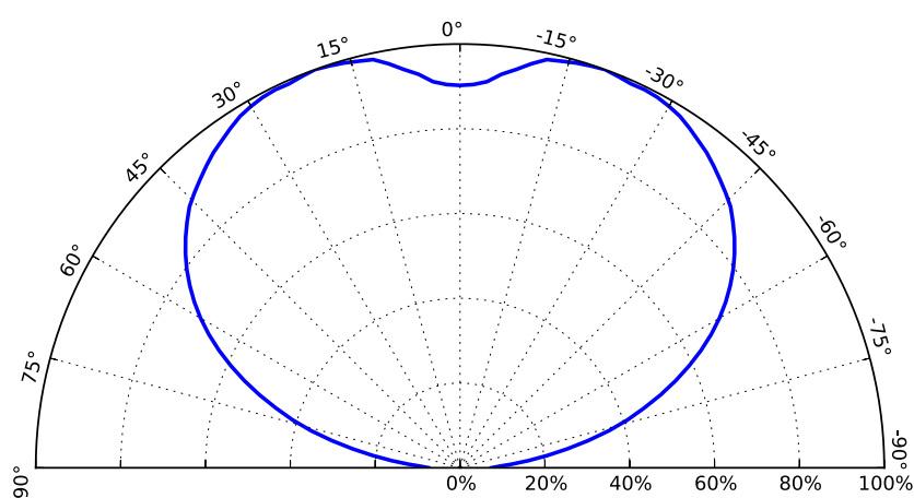
Figure 9. Typical polar radiation pattern for LUXEON UV FC Line at 500mA, T j =25°C.
