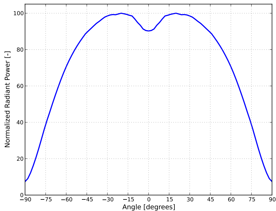
Figure 8. Typical radiation pattern for LUXEON UV FC Line at 500mA, T j =25°C.
