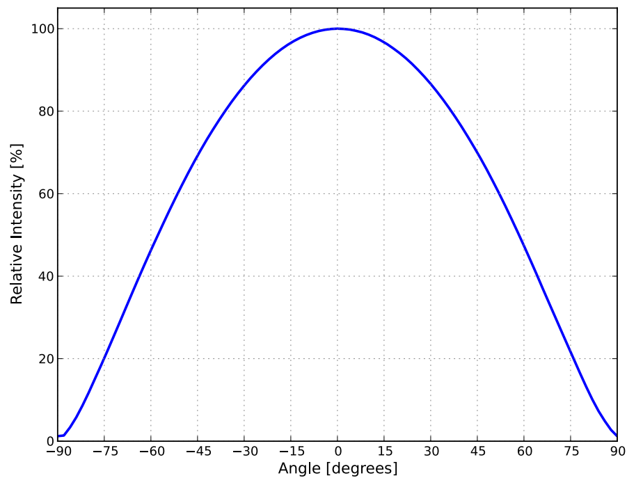
Figure 5. Typical radiation pattern for LUXEON 3014 with FreshFocus Technology at 60mA, T j =25°C.
