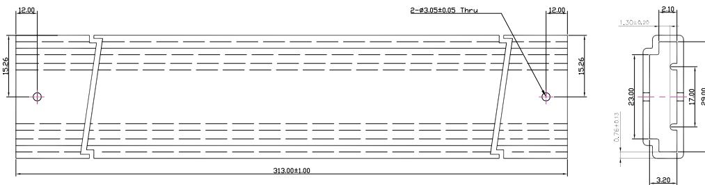
Figure 9b. Tube dimensions for L2C5-xx001211E1900.
