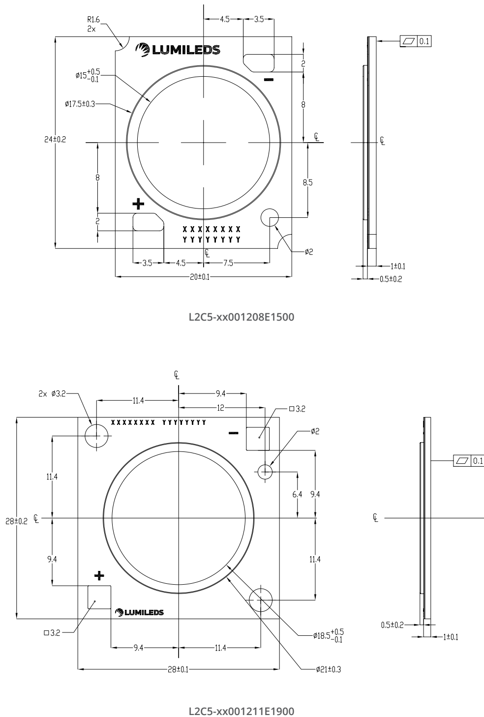
Figure 8. Mechanical dimensions for LUXEON CoB with FreshFocus Technology.
