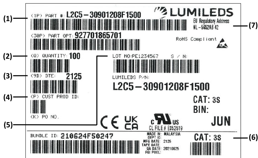
Figure 12. Example of inner box label for LUXEON CoB with FreshFocus Technology.
