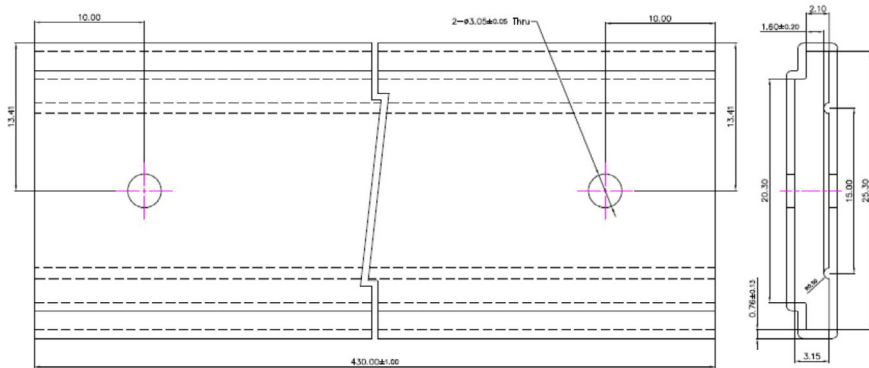
Figure 9a. Tube dimensions for L2C5-xx001208E1500.
