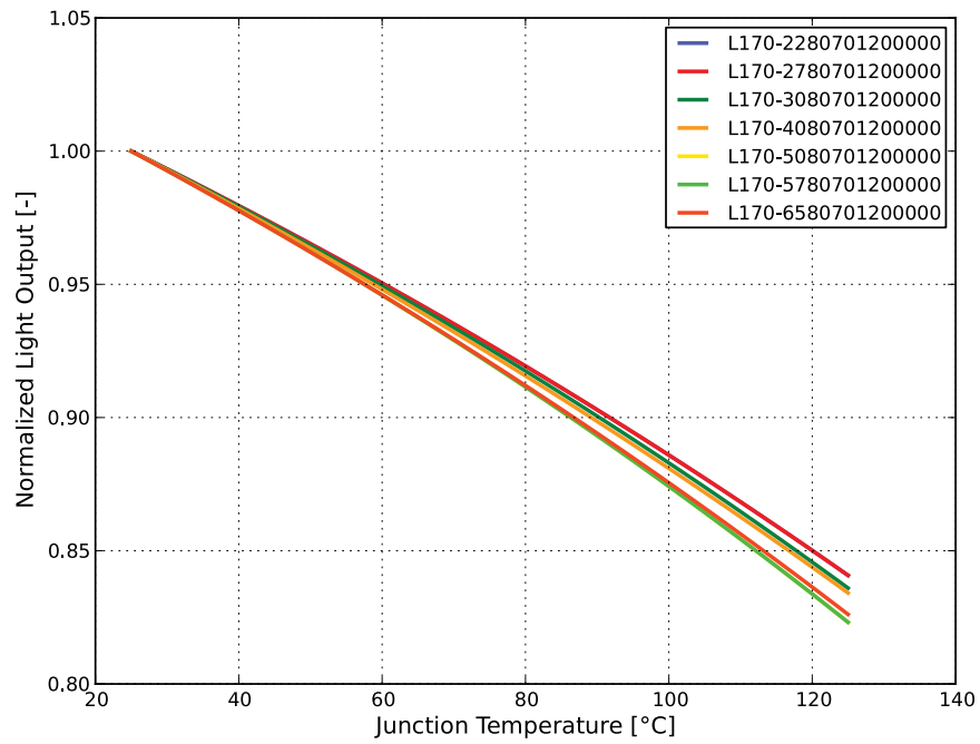
Figure 2b. Typical normalized light output vs. junction temperature for L170-xx80701200000 at test current.
