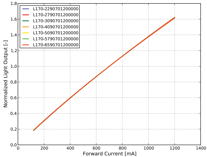
Figure 3c. Typical normalized light output vs. forward current for L170-xx90701200000, T_j = 25^\circ\text{C} .
