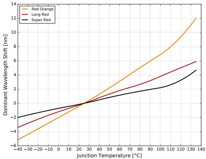
Figure 1b. Typical wavelength shift vs junction temperature for SignalSure 250 at 20ms MP, 250mA, T_j=25^{\circ}\text{C} .
