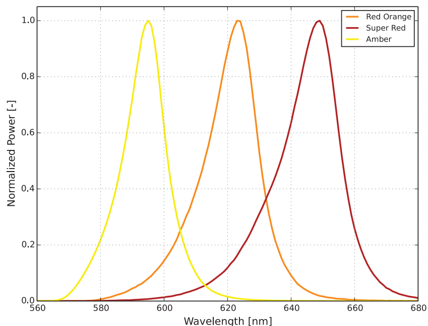
Figure 1. Typical normalized power vs. wavelength for SignalSure 150 at 20ms MP, 150mA, T_j=25^{\circ}\text{C} .
