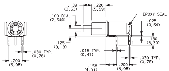
TP12SH9ABE SPDT
