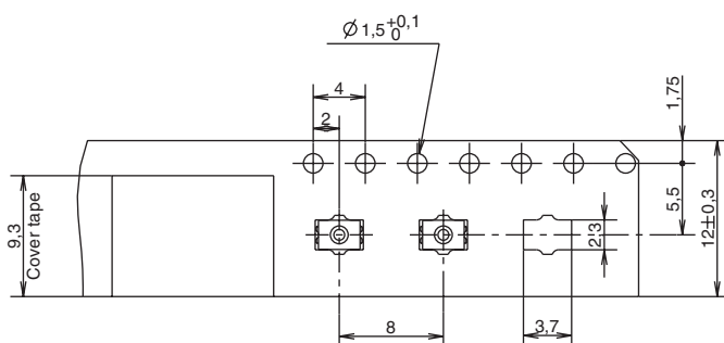
CARRIER TAPE
