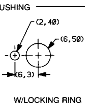
W/LOCKING RING
