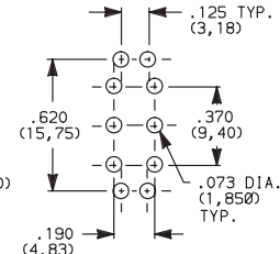
PC MOUNTING
