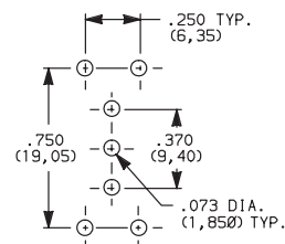
PC MOUNTING
