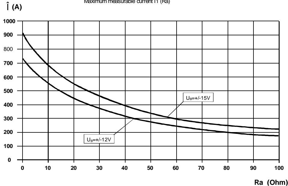
Maximal meßbarer Strom \hat{I}_1 ( R_a ) Maximum measurable current \hat{I}_1 ( R_a )
