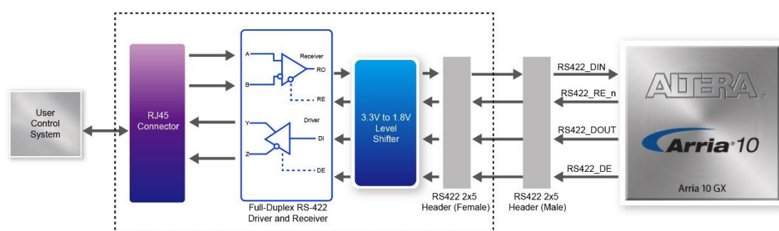
Figure 2-14 Block Diagram of RS-422 application
