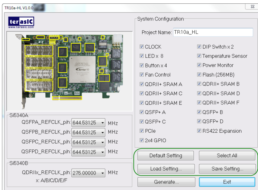
Figure 3-6 Project Settings
