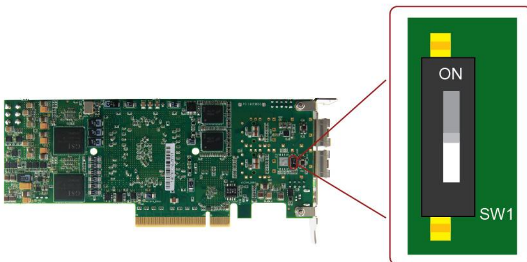
Figure 2-4 Position Dip Switch for FPGA Configuration
