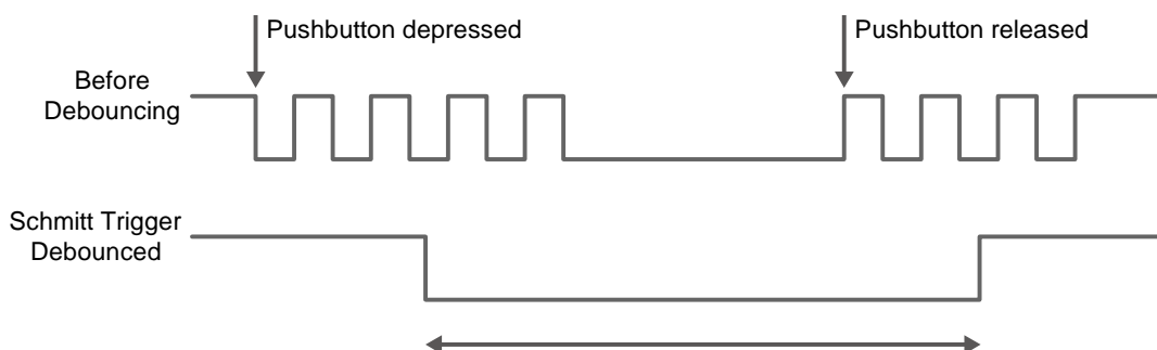
Figure 4-7 Switch debouncing
