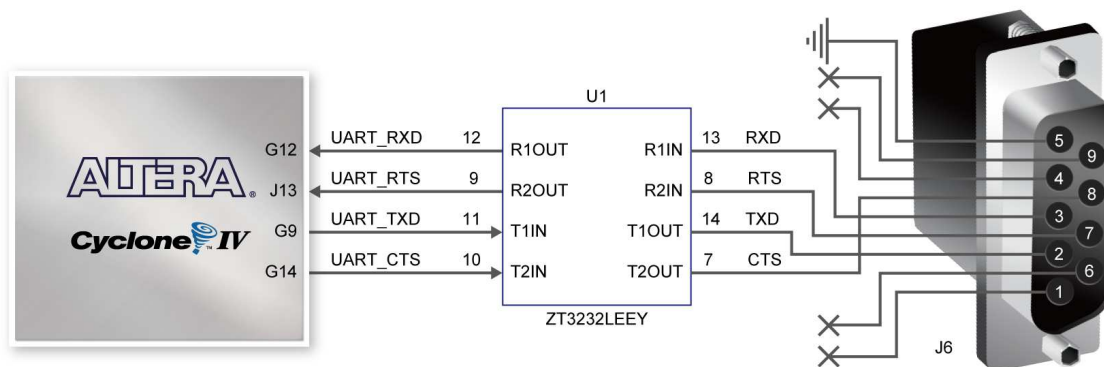
Figure 4-24 Connections between FPGA and ZT3232 (RS-232) chip
