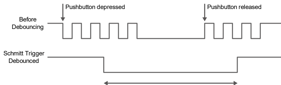
Figure 3-15 Switch debouncing
