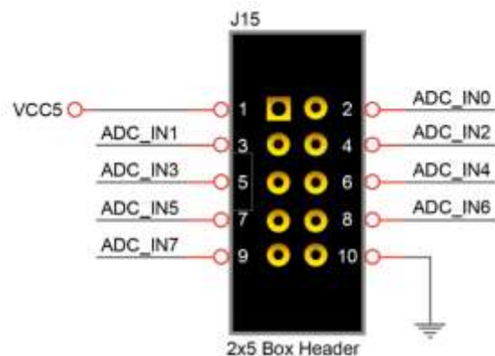
Figure 5-22 Pin distribution of the 2x5 Header for the ADC
