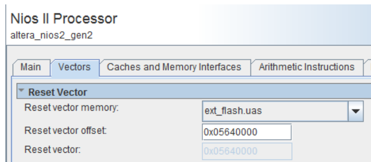
Figure 4-7 Factory Software Reset Vector Settings for NIOS II Processor
