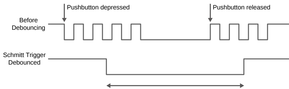
Figure 4-6 Switch debouncing
