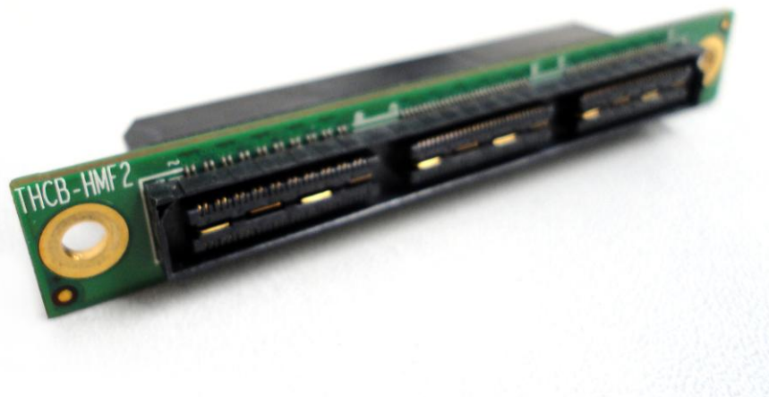
Figure 1-3 THCB-HMF2 card
