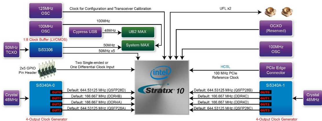
Figure 2-11 Clock circuit of the FPGA Board
