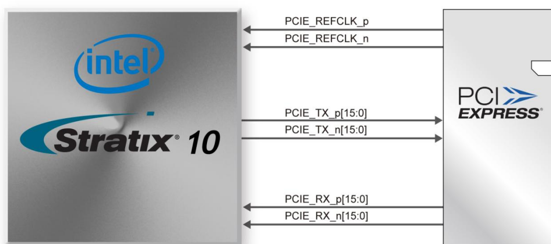
Figure 2-16 PCI Express pin connection
