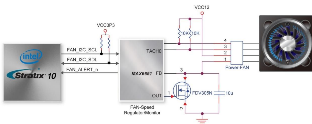
Figure 2-9 Connections between the Fan-Speed Regulator/ Monitor and the Stratix 10 GX/SX FPGA
