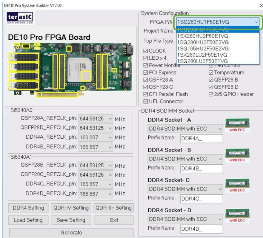
Figure 3-3 Select FPGA
