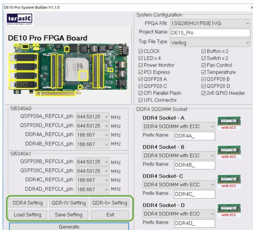
Figure 3-8 Project Settings
