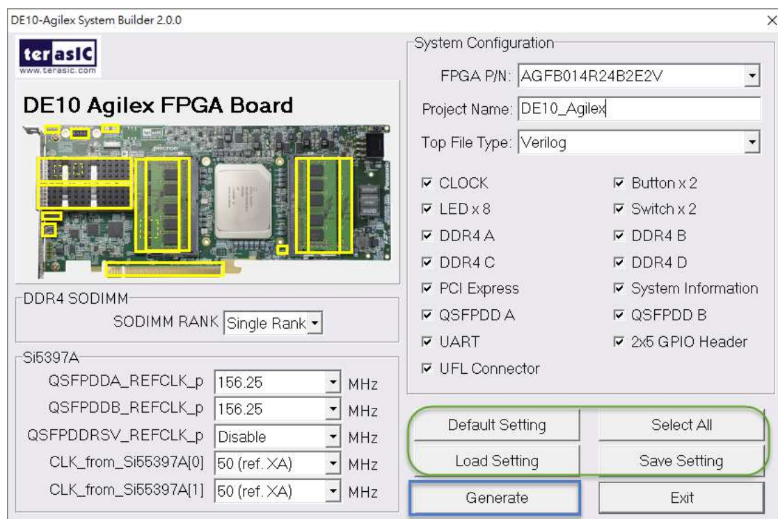
Figure 3-11 Project Settings
