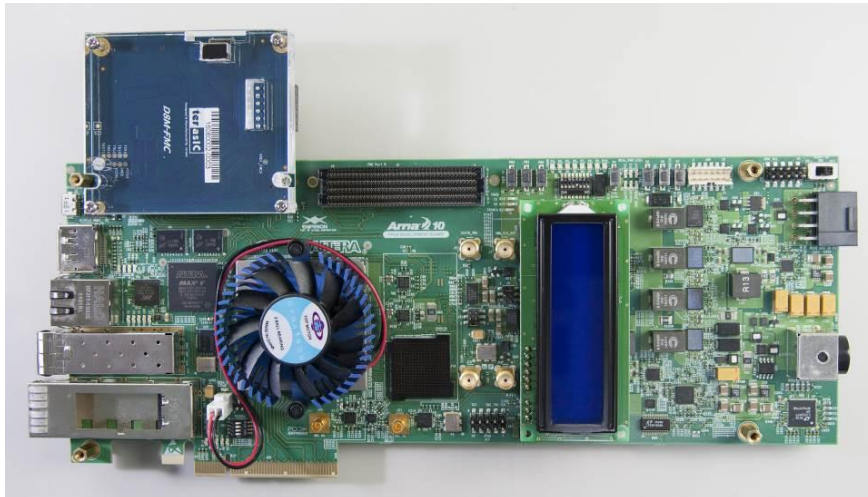
Figure 1-4 Connect the D8M-FMC to A10GFP board's expansion port
