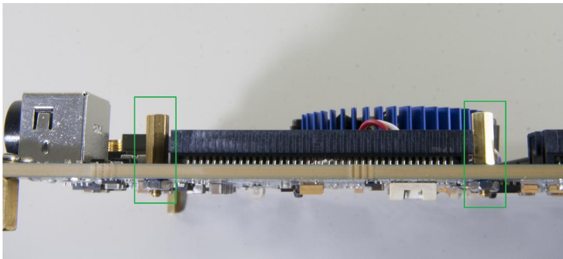
Figure 1-6 Mount the copper pillar to the TR5 Board
