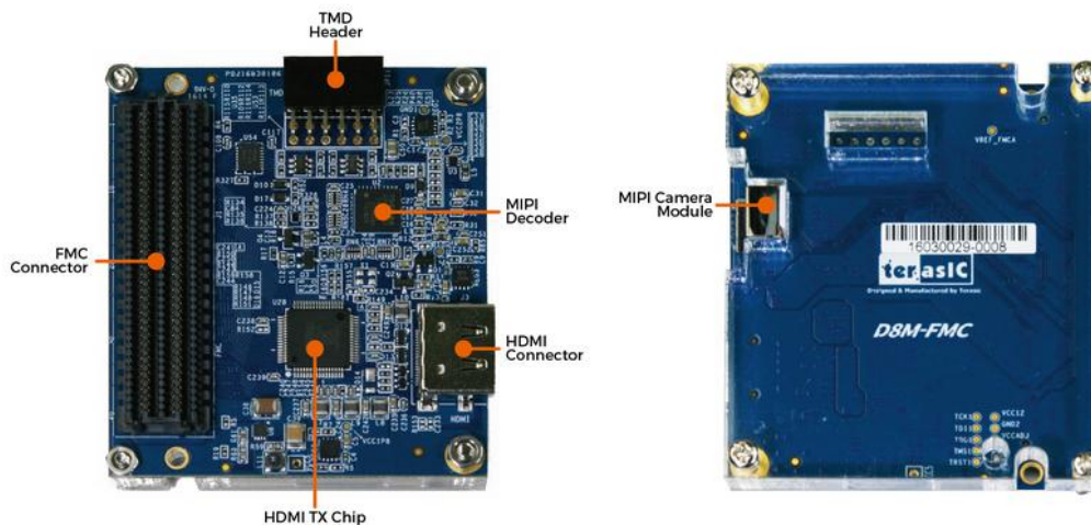
Figure 2-1 D8M-FMC Board
