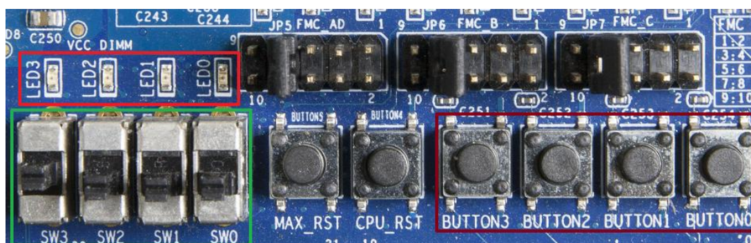
Figure 4-3 Buttons/Swtiches/LEDs on TR5 Board
