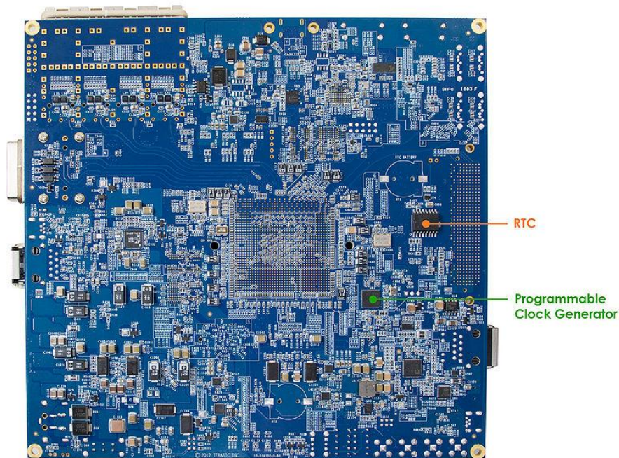
Figure 2-2 HAN Pilot Platform (bottom view)
