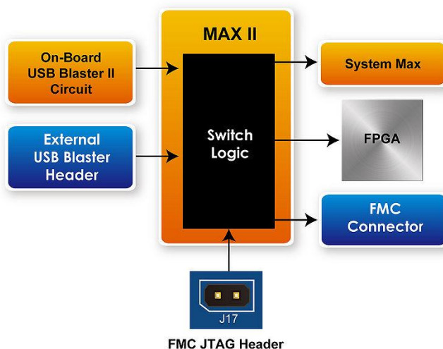
Figure 3-7 JTAG interface of HAN Pilot Platform
