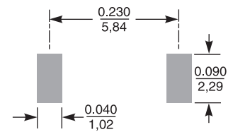
Recommended Land Pattern
