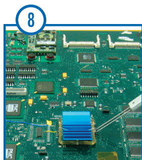
Using the "Forked End" of the Spring Clip tool, "latch over" the "Closed End" of the Spring Clip on to the Frame Clip tab.
