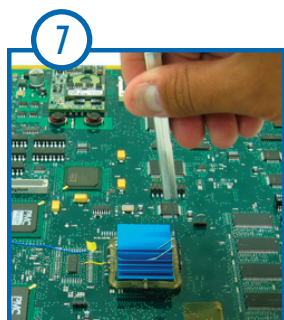
Secure the "Open End" of the Spring Clip under the lip of the frame clip.
