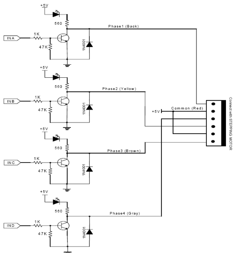
FIG 2: MR-MINI-STEP-MOTOR Schematic
